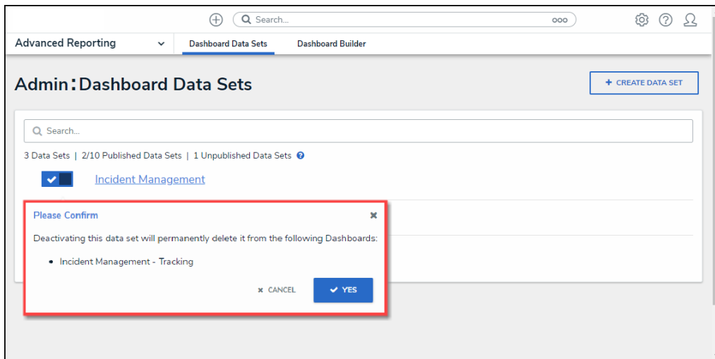
Confirmation Pop-up
