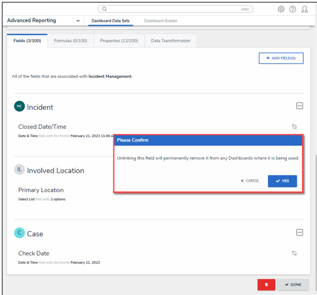
Confirmation Pop-up
